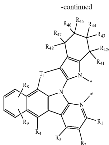
Formula 4-74
