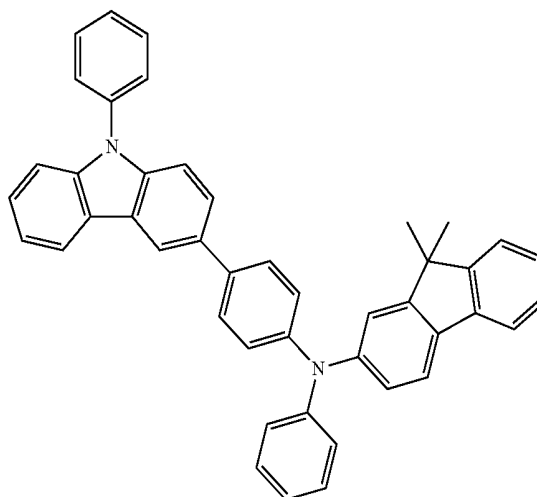
HT1
