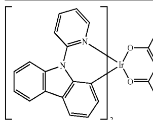
Comparative Compound 1
