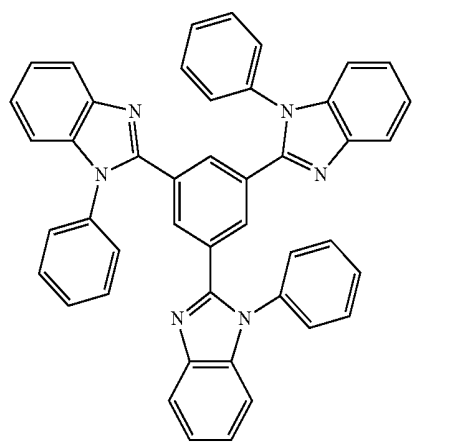
TPBi
