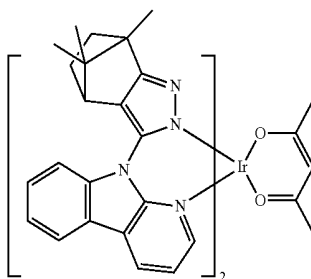
Compound 9
