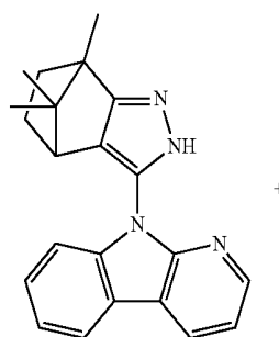
Compound A
